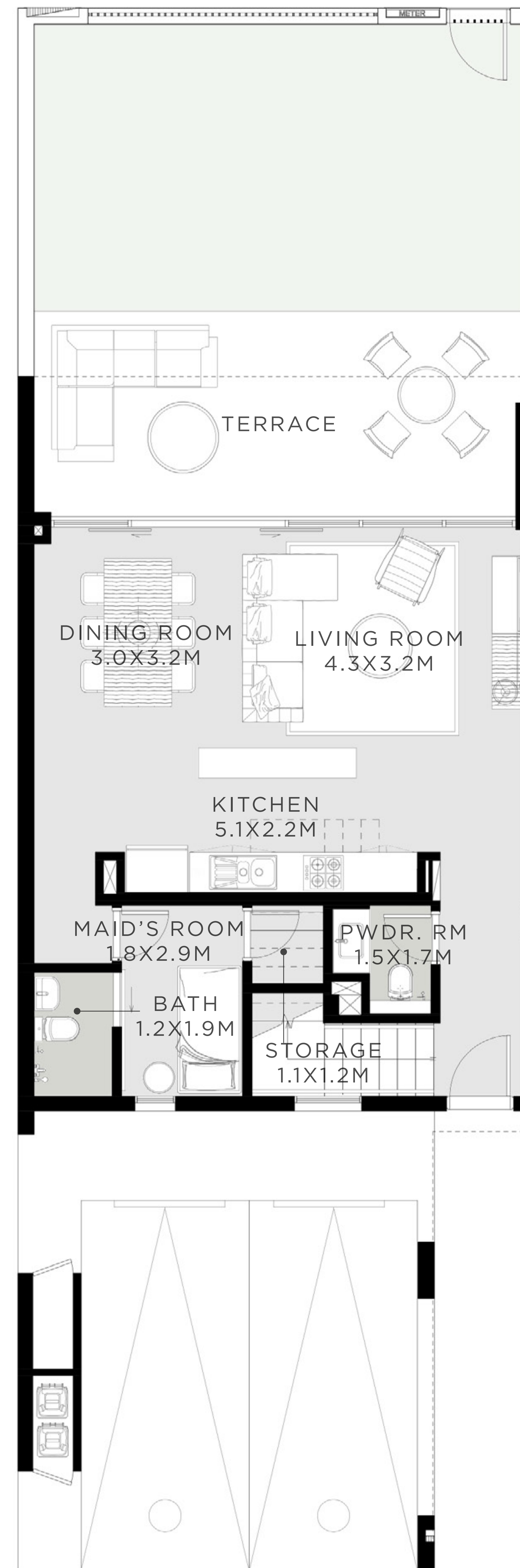
GROUND FLOOR
