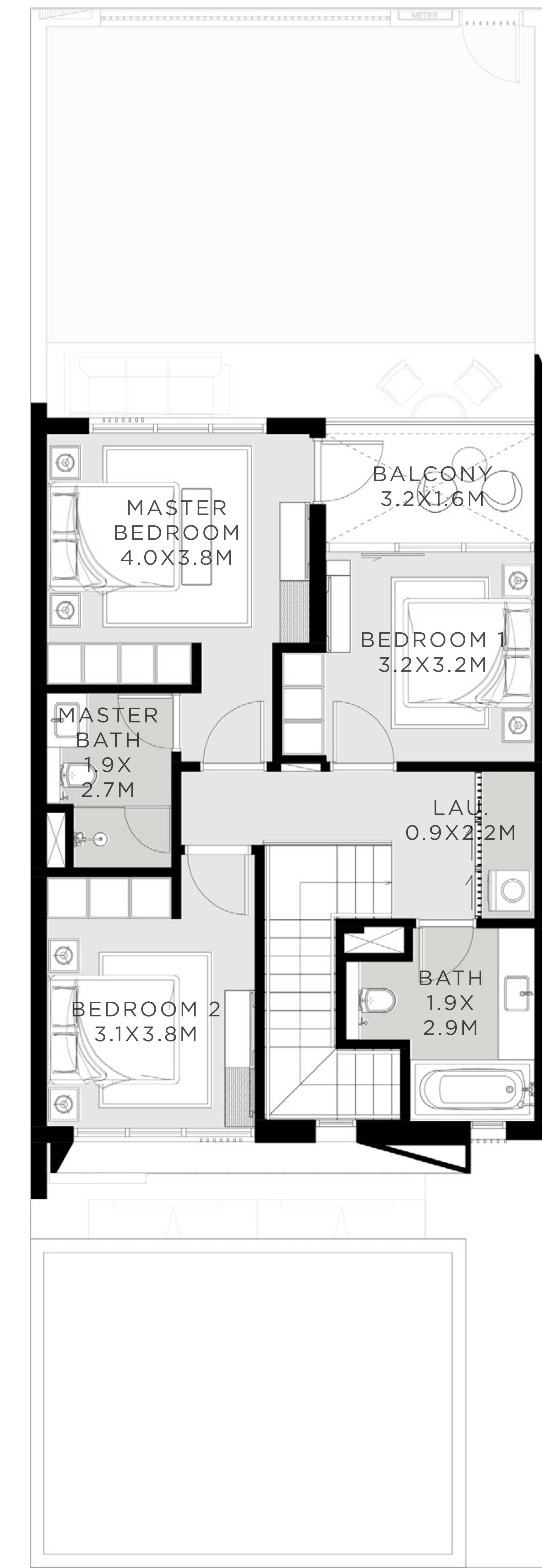
FIRST FLOOR
